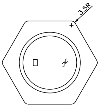
VIEW ON BASE SHOWING EMBOSSED MARKING
