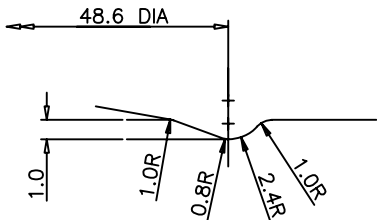
STACKING RING DETAIL SCALE 5:1
